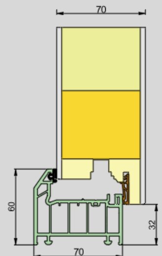
Option 3 60mm PVC Wraparound Threshold
