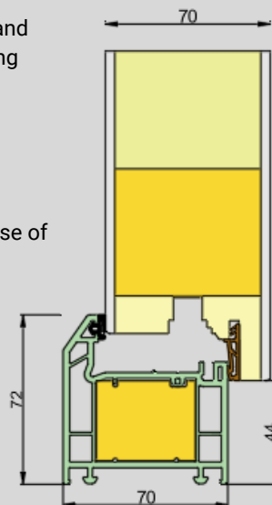
Option 2 72mm PVC Wraparound Threshold
